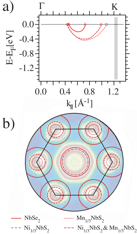
Fig. 3. Comparison between the Nb 4d band filling of NbSe 2 , Mn 1/3 NbS 2 and Ni 1/3 NbS 2 . (a) Summary of the dispersion maps from Figure 1a. Note the two positions of the K point due to the variation in lattice constant during intercalation. (b) Sketch of the effect of doping on the Fermi surface.
